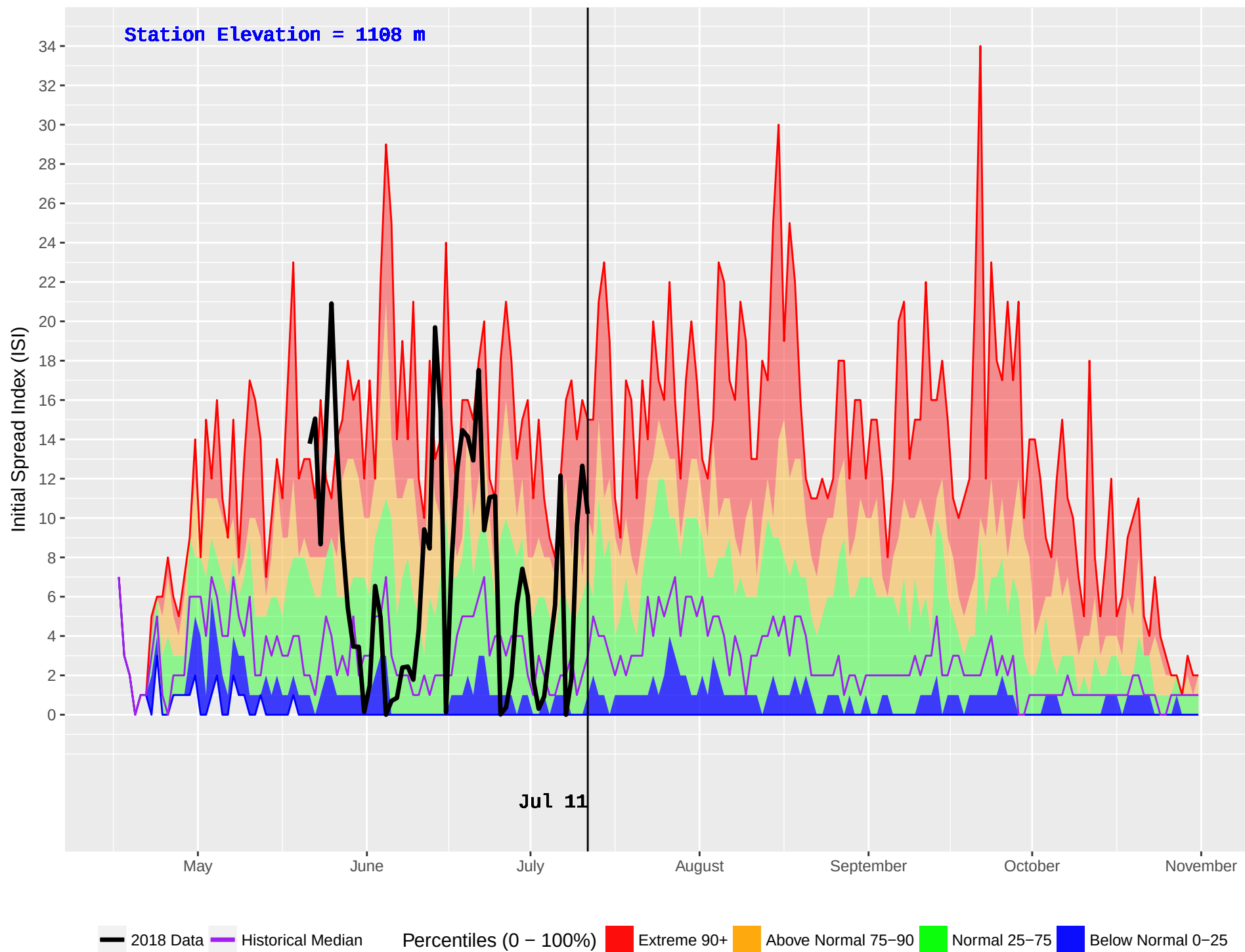
NABESHE (151) : Historical (1987–2016) and Current (2018) Noon Initial Spread Index (ISI)
